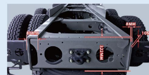
Reinforced Frame Chassis [10+8mm]
